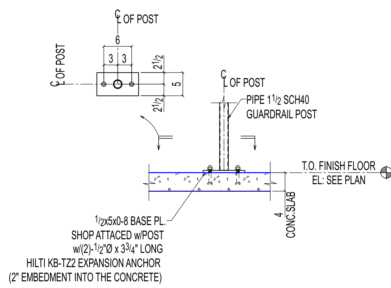
4 DETAIL SE707 (OTHERS NOT SHOWN FOR CLARITY)
