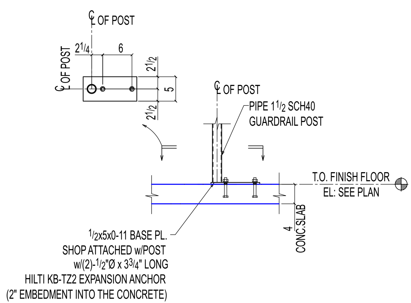
3 DETAIL SE707 (OTHERS NOT SHOWN FOR CLARITY)
